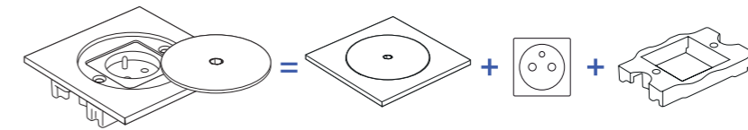
Secured opening lid + mechanism + mechanism support
